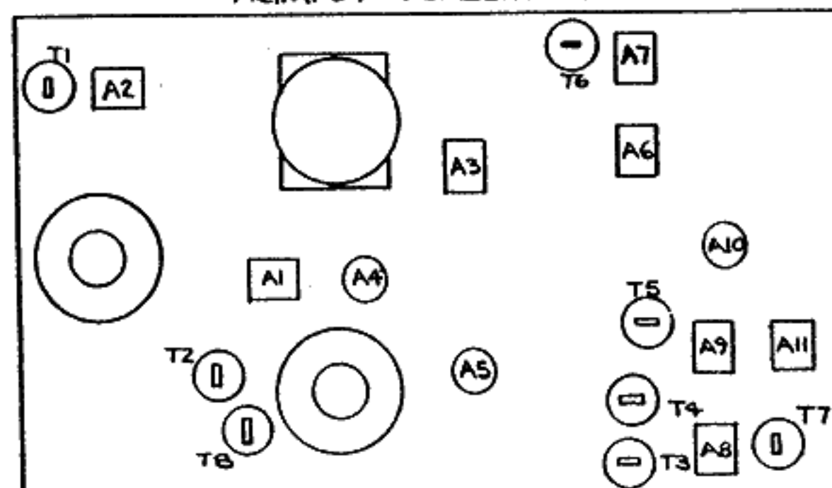
TRIMPOT PLACEMENT
